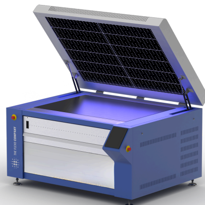
Xpro M-ELF Exposure LED + Flouorescent Lamps Light Finisher
